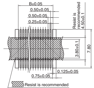
Recommended PC board pattern (TOP VIEW)
